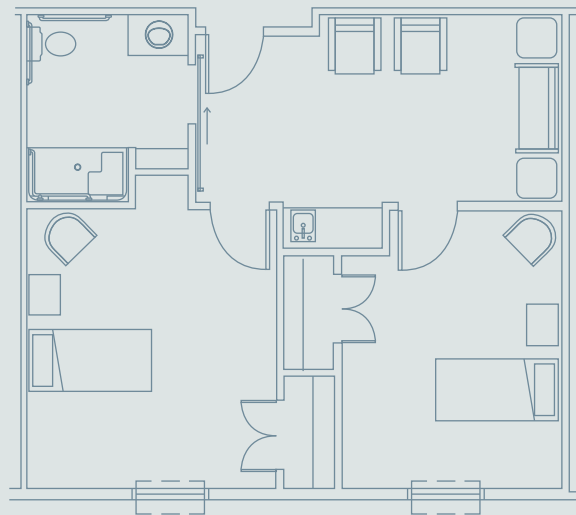
TWO BEDROOM UNIT 688 Sq. Ft.
